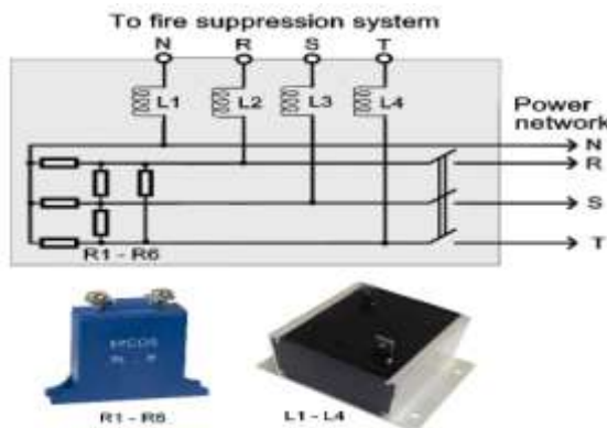
Fig.+ 11 Design and components of a filter for power circuits of powerful automatic fire extinguishing control systems. R1-R6 –varistor blocks; L1-L4 – special chokes.
