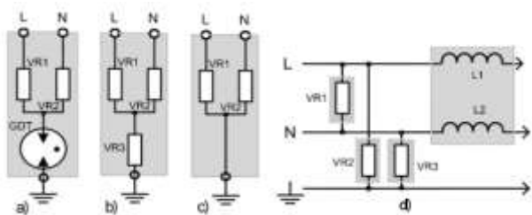
Fig. 9 Various protection units (a, b, c) and suggested connection of protection elements (d). VR1 – VR3 – metal-oxide varistors (MOV); GDT – gas discharge tube; L1 – L2 – current-limiting chokes.
